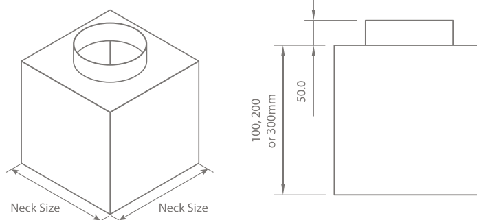
Top Entry
