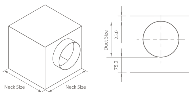
Side Entry
